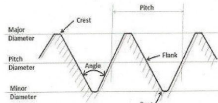
Basic Thread Terms
